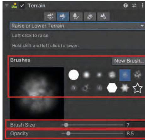
Görsel 1.57: Brushes, Brush Size ve Opacity
